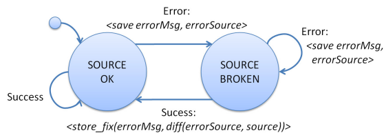
Figure 6. A state machine tracks compiler errors to collect fix reports for the HelpMeOut database. Error connotes a failed compilation, Success a successful compilation.
