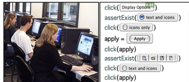
Figure 1. GUI testing (left) traditionally requires human testers to operate the GUI and verify its behavior visually. Our new testing framework allows the testers to write visual scripts (right) to automate this labor-intensive task.
