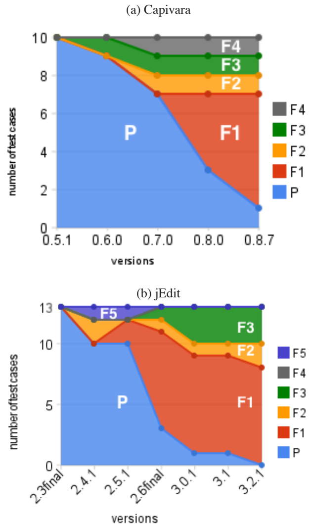
Figure 6. Long-term regression testing.
