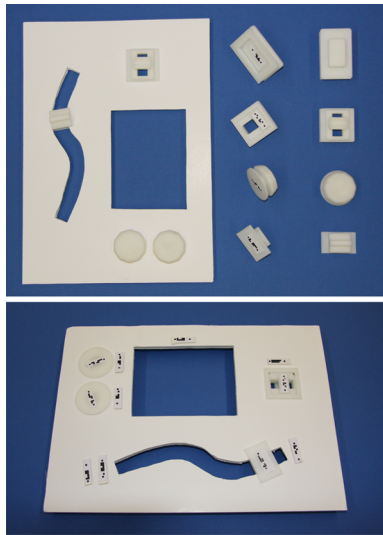
Figure 5: Top : Example of a designed front panel made of foam board and 3D printed controls.
