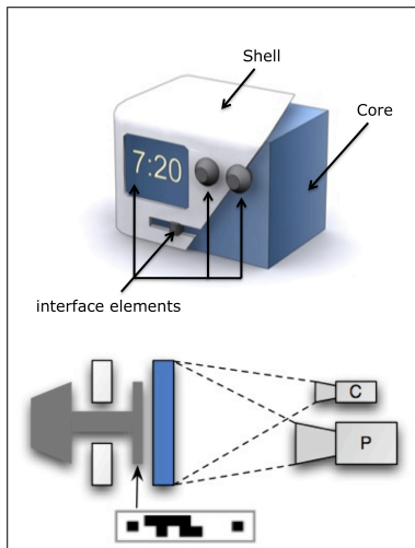
Figure 3: Example device with white cut-out Shell and blue Core (top), and side view (bottom) with dark-grey control, attached visual code, camera (C) and projector (P).
