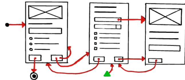
Figure 3: An Example of the complete visual input for developing a mobile application. The sketch includes all screens and the main application flow.
